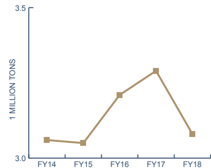
CHART 2.7: MSW Disposed Of
