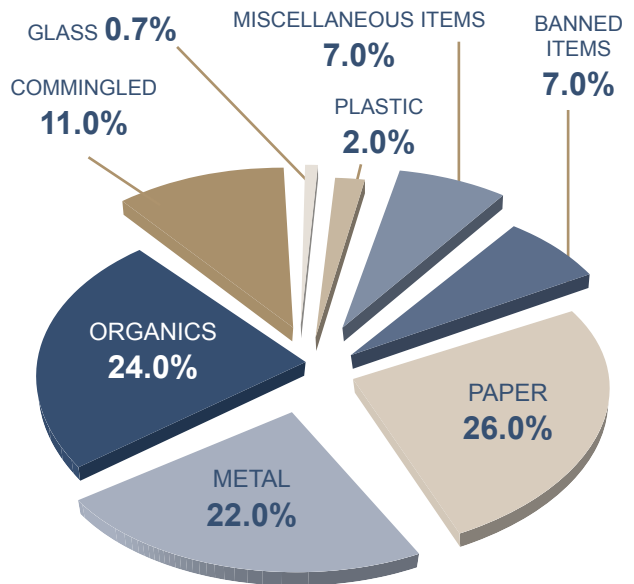
CHART 4.2: MSW Commodities Recycled as a Percentage of All MSW Recycled in FY18
