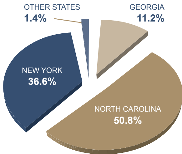
CHART 7.3: Percentage of All Solid Waste Imported into South Carolina by State in FY18
