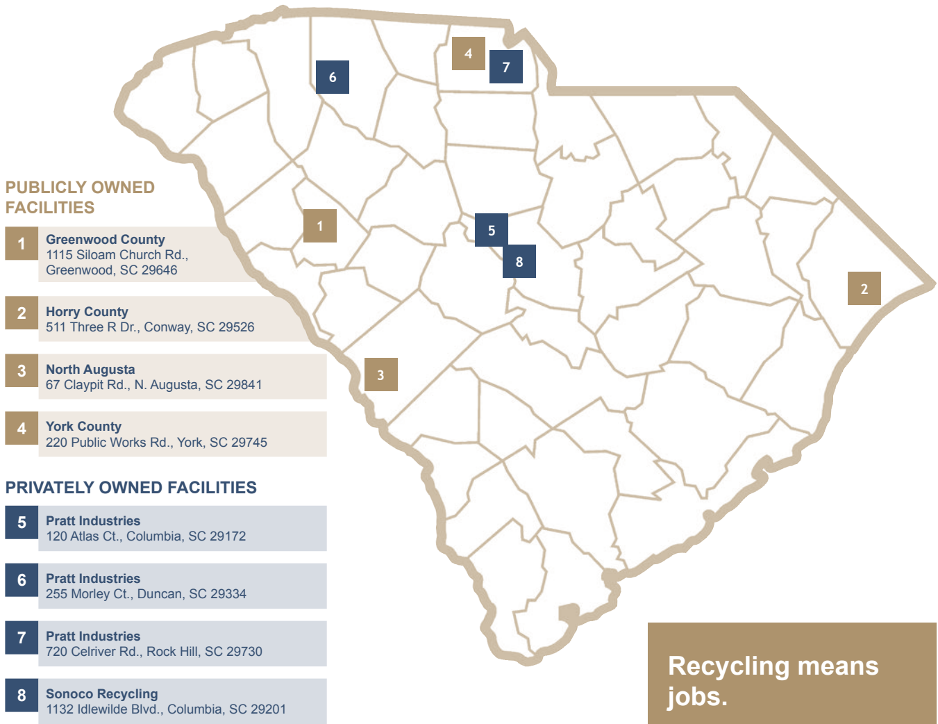
FIGURE 3.1: South Carolina's Materials Recovery Facilities in FY18
