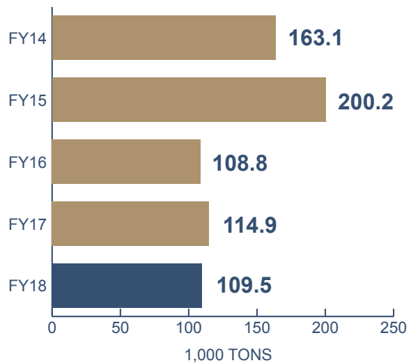
CHART 7.4: Tons of All Solid Waste Exported from South Carolina in FY18
